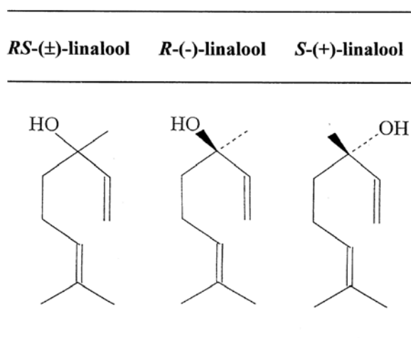
Figure 9. Formulas of the enantiomeric isomers of linalool.
